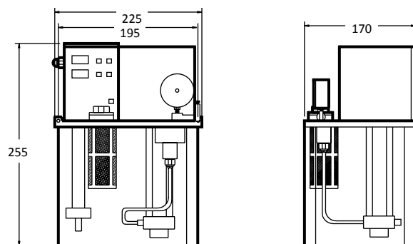
3 Liter Reservoir
